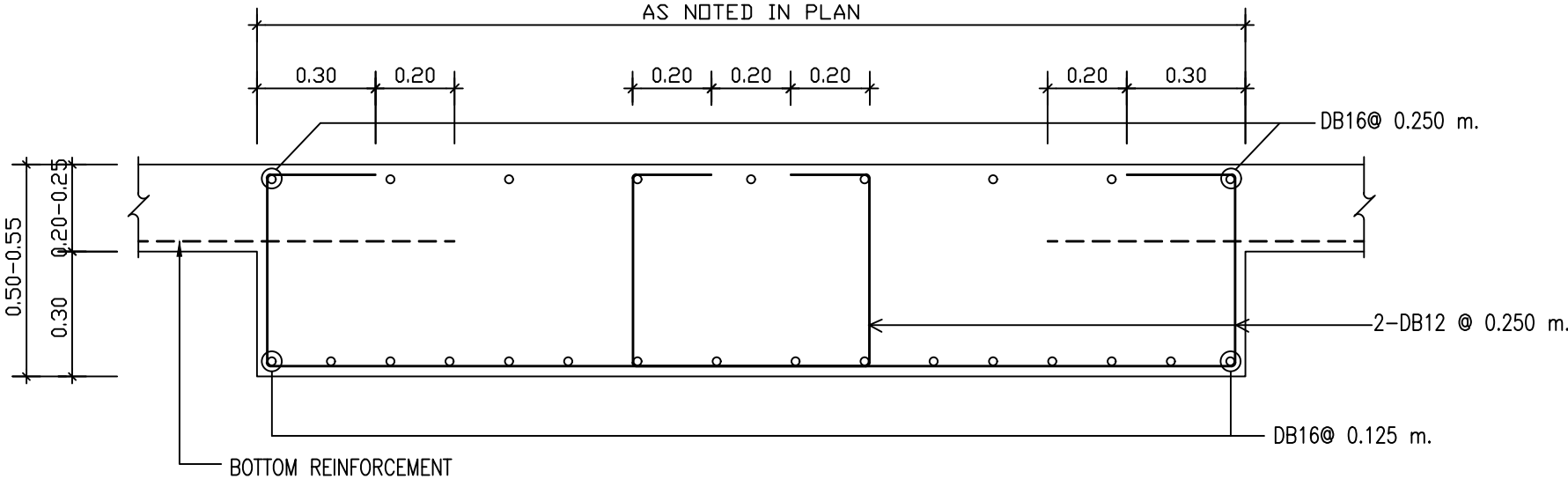
PB2 0.50-0.55 M.THK. (T-SHAPE)
