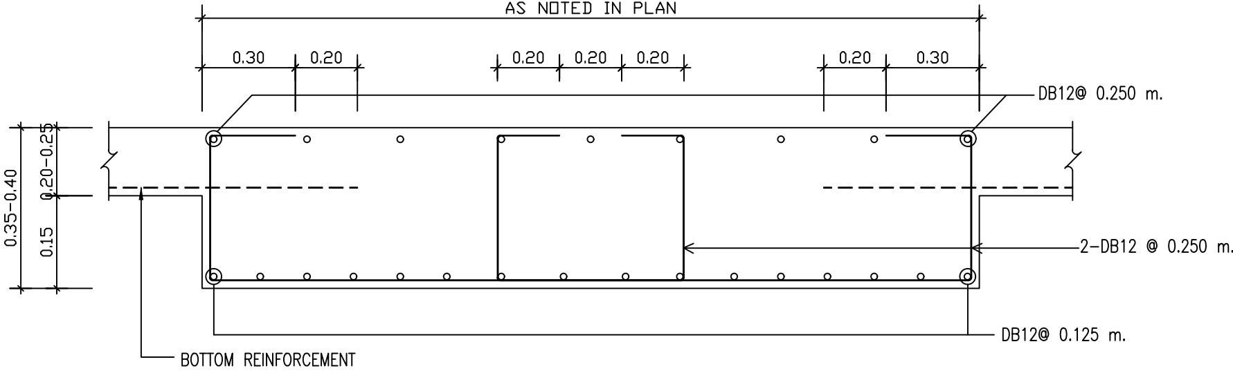
PB1 0.35-0.40 M.THK. (T-SHAPE)
