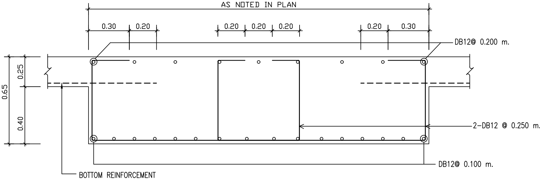
PB3 0.65 M.THK. (T-SHAPE)
