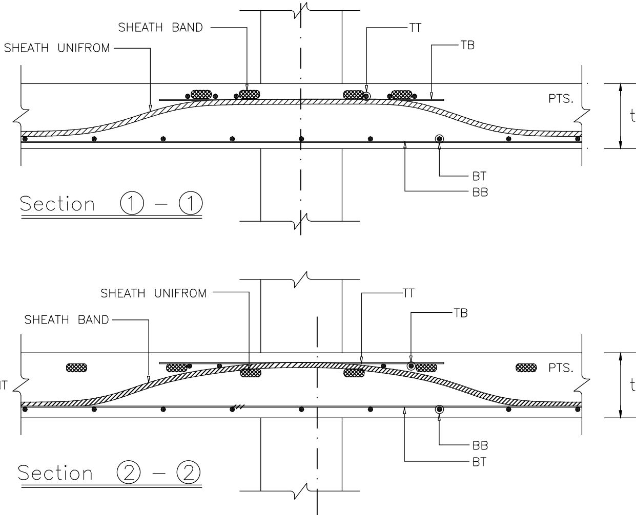
12. TYP. REINFORCEMENT AT COLUMN
