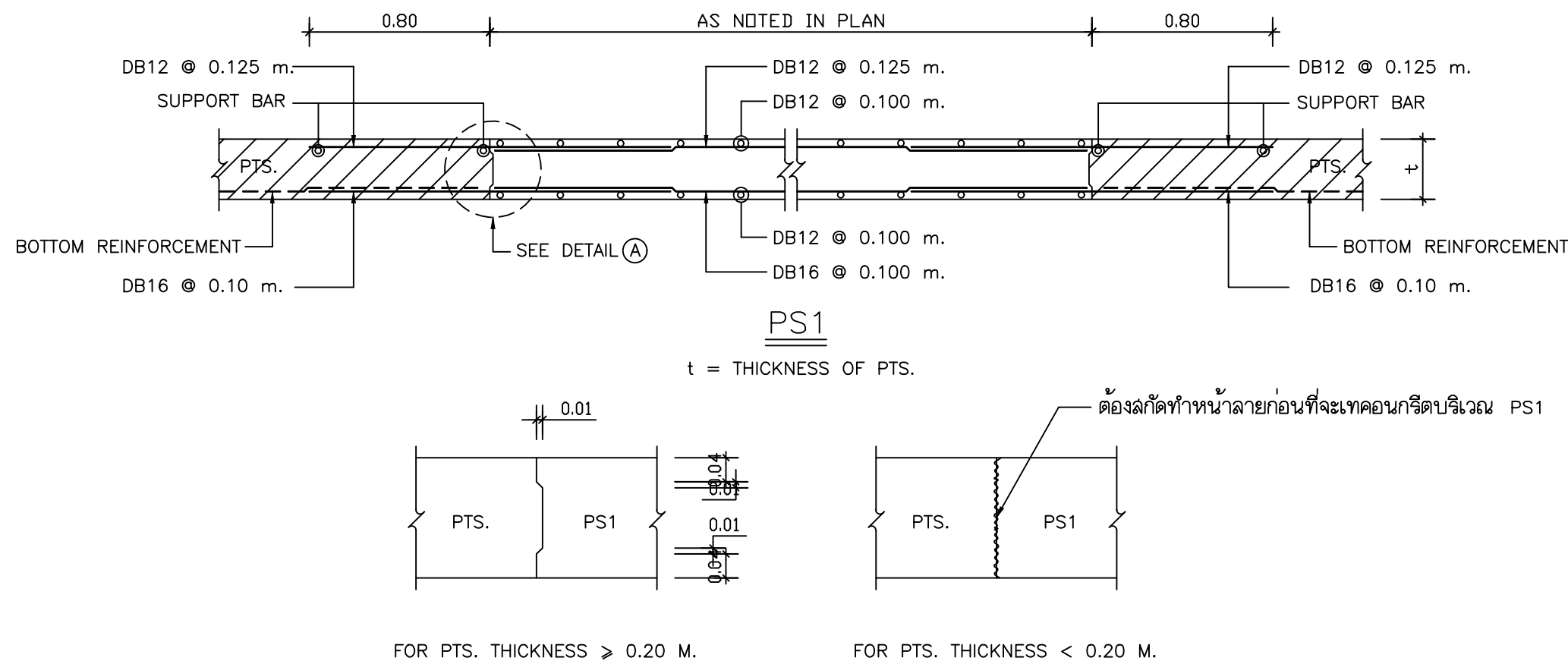
DETAIL (A)
