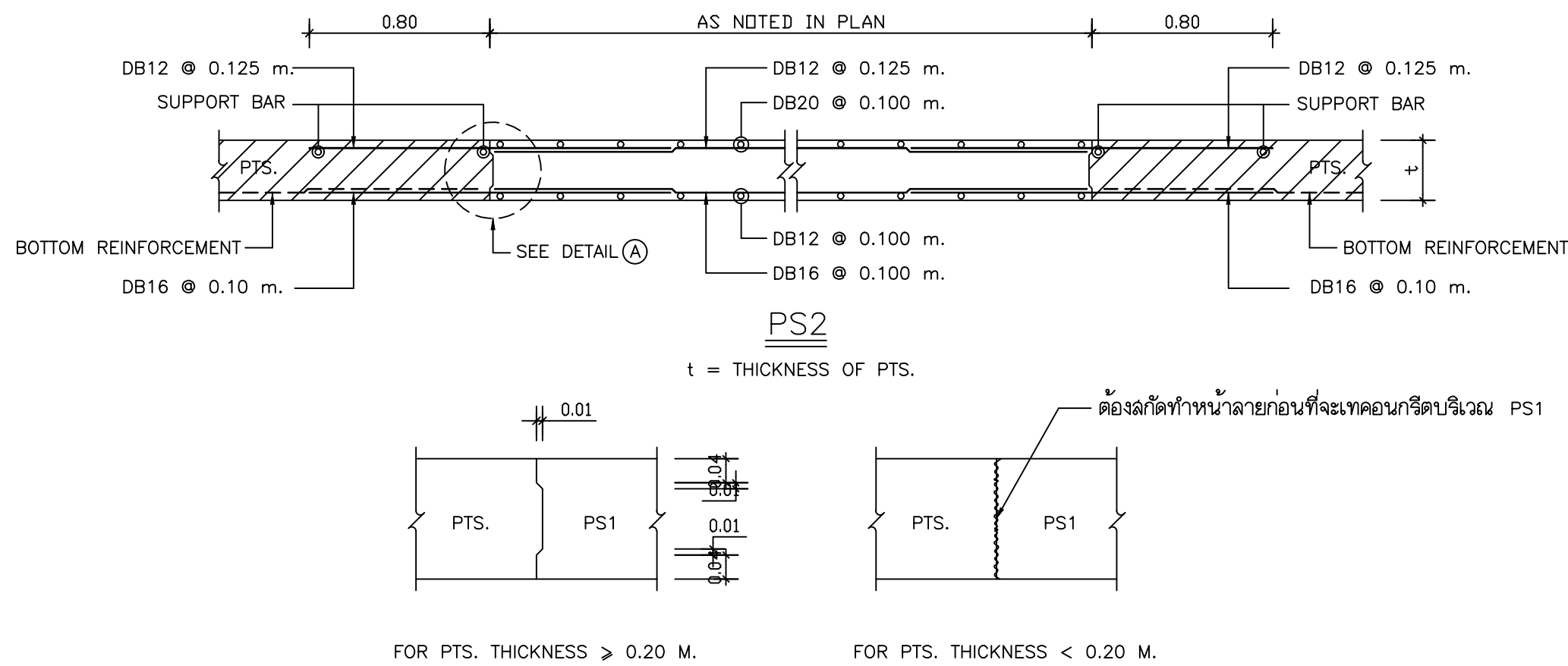
DETAIL (A)
