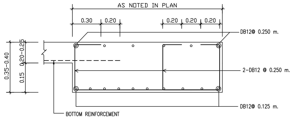
PB1 0.35-0.40 M.THK. (L-SHAPE)
